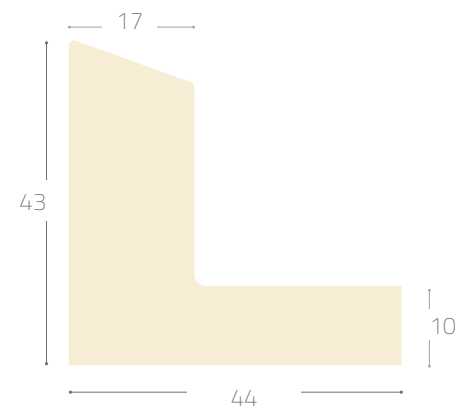
Profile 3761#
