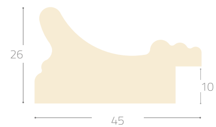
Profile 3175#
