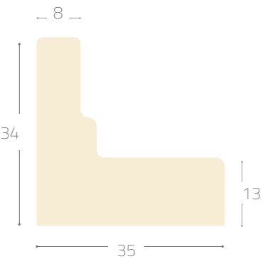
Profile 3304#
