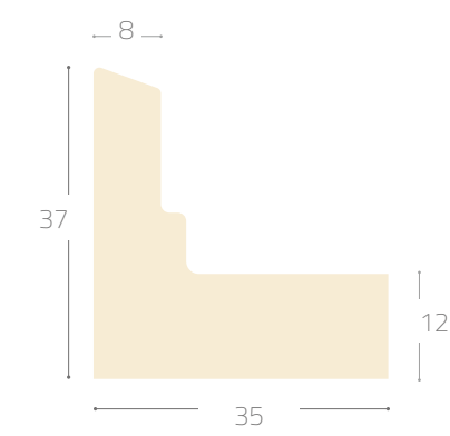
Profile 3760#
