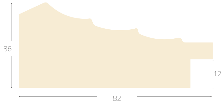
Profile 1181#
