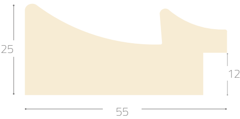
Profile 1775#
