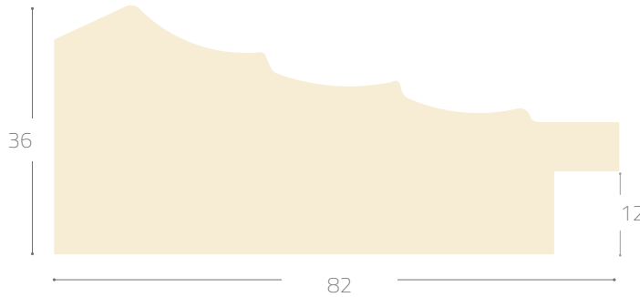
Profile 1181#
