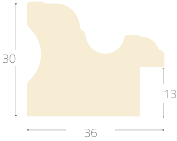
Profile 3176-A#
