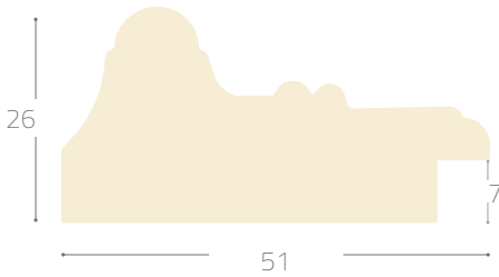
Profile 3341#
