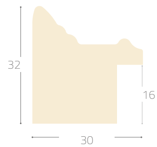
Profile 3752#
