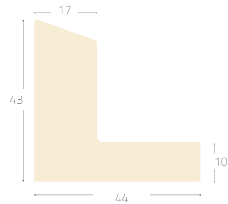
Profile 3761#
