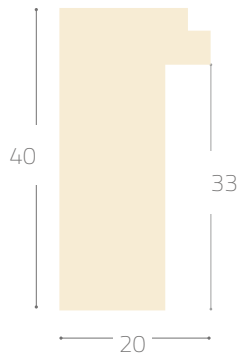
Profile 3758#
